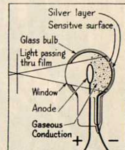
Fig. 2—Action of photo-electric cell light entering cell through window. Current can flow.
